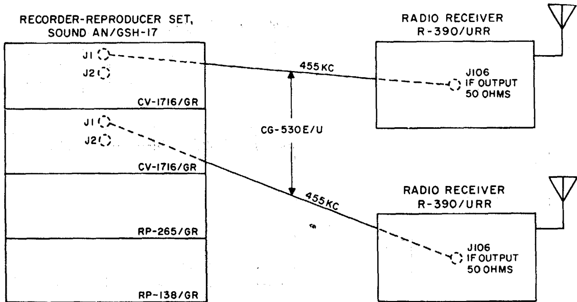
Figure 2-7. Setup for receiving coder-burst transmission for a premission equipment check.
