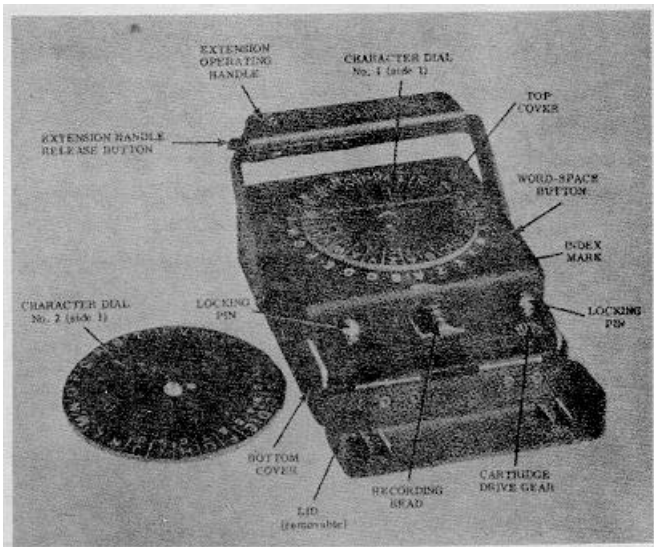
Figure 1-2. CO/B-8 Coder.
