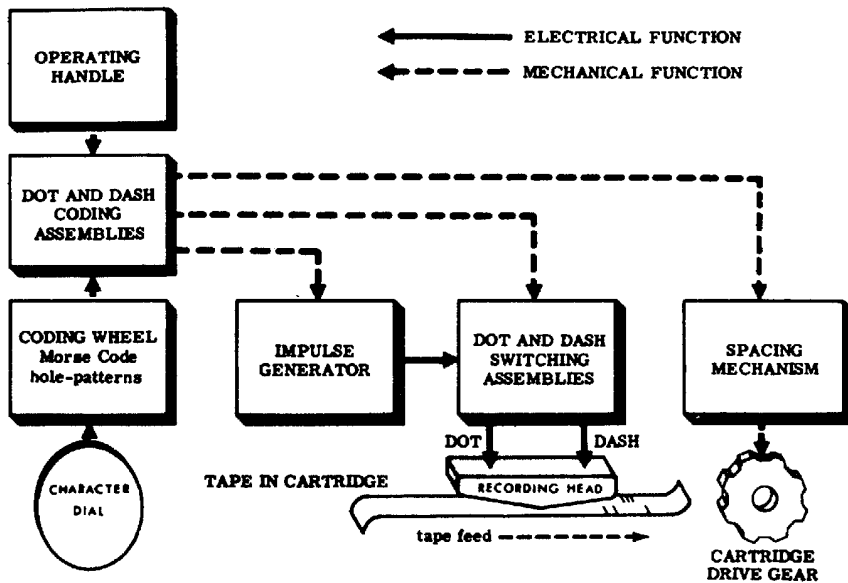
Figure 3-3. CO/B-8 Coder functional block diagram.
