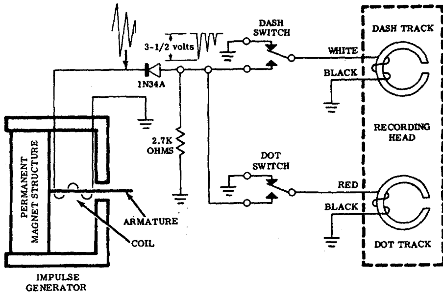
Figure 4-3. Impulse generator diagram for CO/B-8 and CO-3B Coders.
