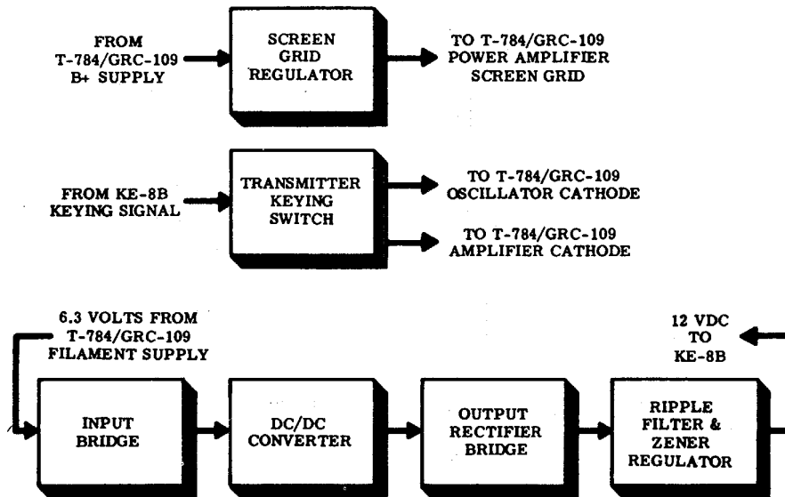
Figure 3-9. KA-3 Keyer Adapter functional block diagram
