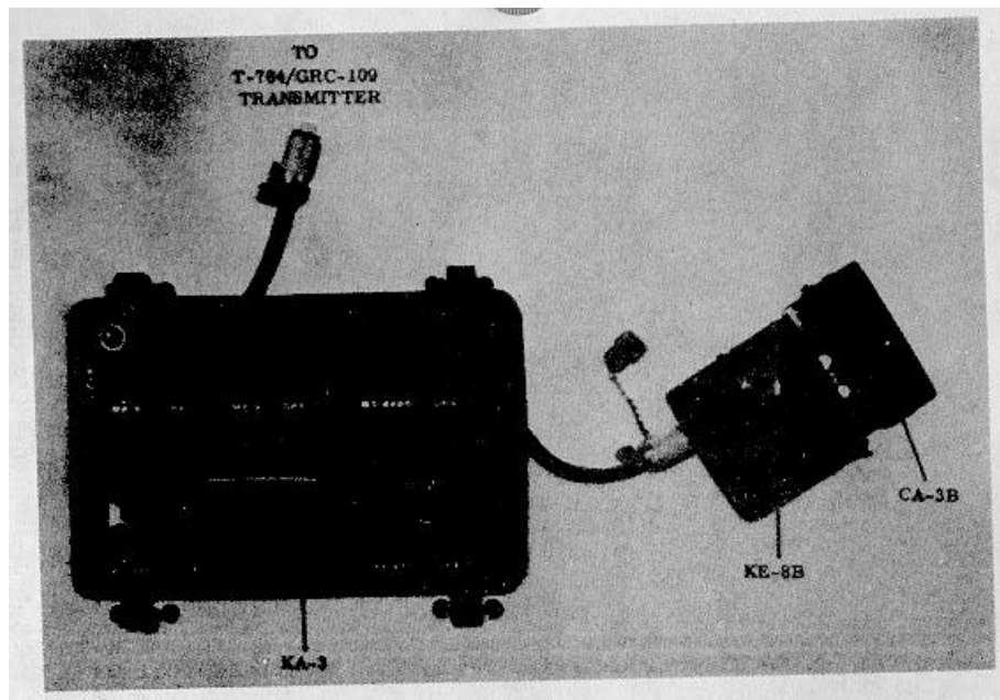
Figure 2-4. KE-3B Keyer connection to KA-3 Keyer Adapter.
