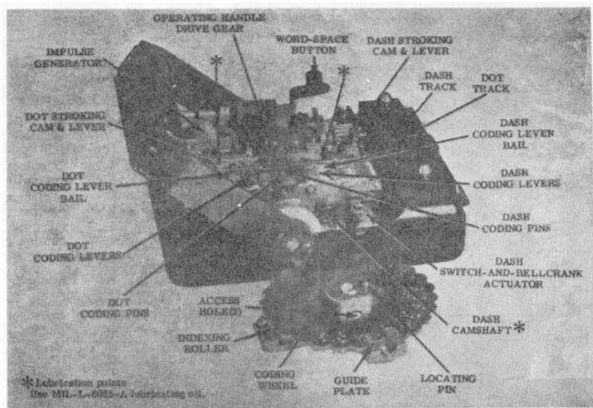
Figure 3-4. CO/B-8 Coder internal mechanism.
