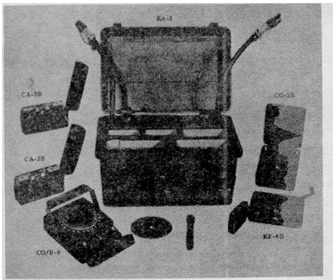
Figure 1-1. AN/GRA-71 Coder-Burst transmission group components.
