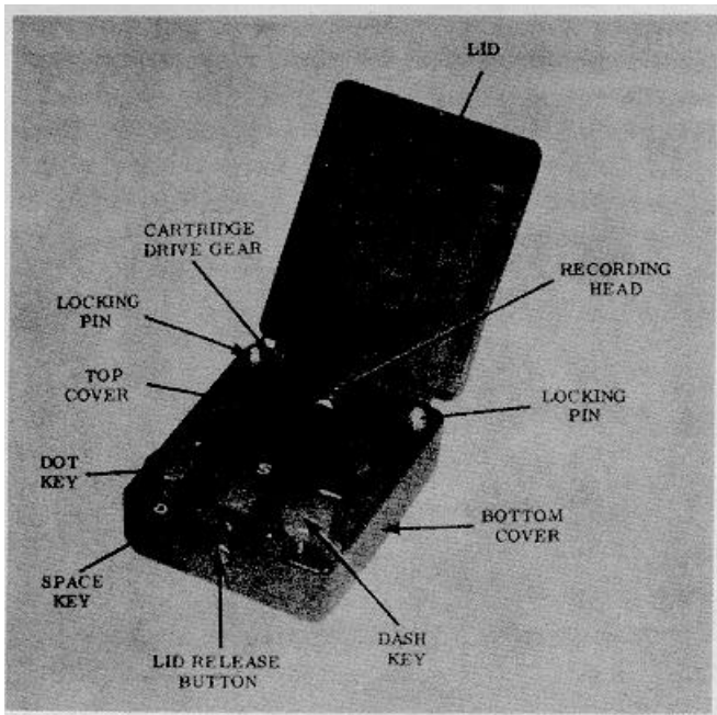
Figure 1-3. CO/3B Coder.
