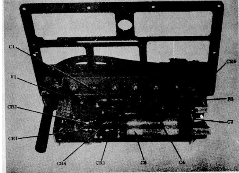
Figure 4-10. KA-3 Keyer Adapter electronics chassis, bottom view.
