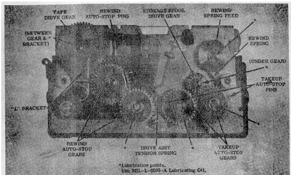
Figure 3-8. CA-3B Cartridge internal mechanism.
