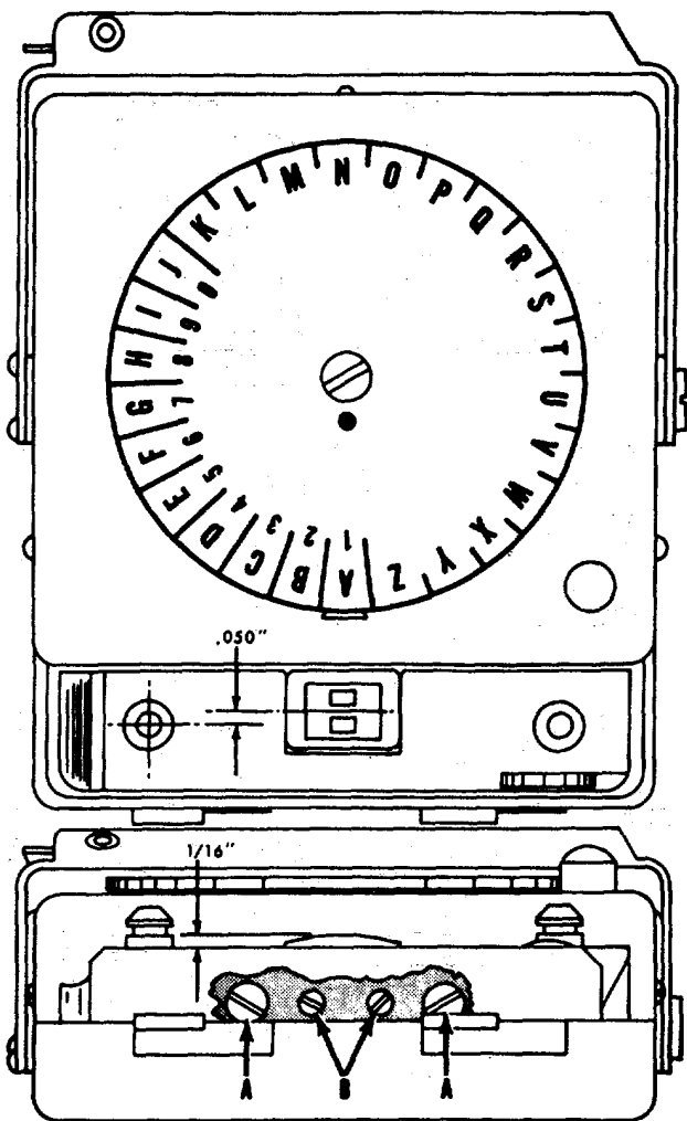
Figure 4-4. CO/B-8 Coder recording head alignment.
