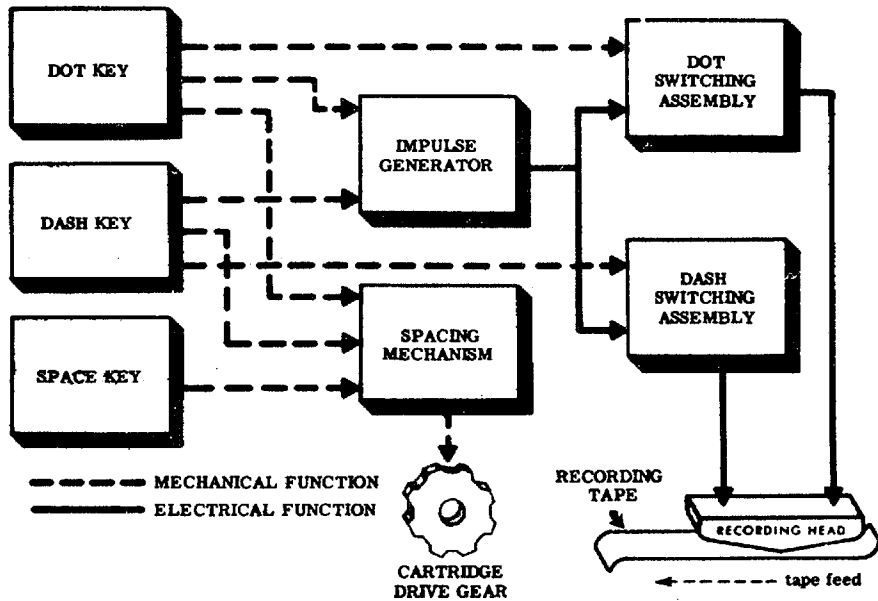
Figure 3-5. CO-3B Coder functional block diagram.
