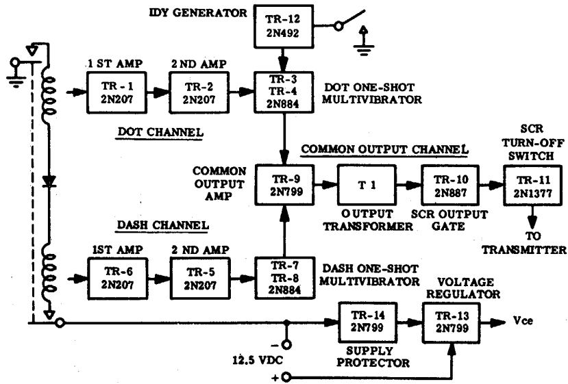
Figure 3-7. KE-8B Keyer electronics section functional block diagram.
