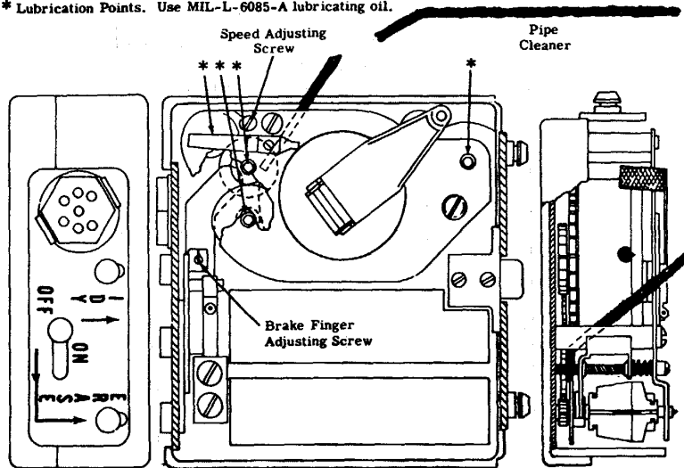
Figure 4-6. KE-8B Keyer brake disc cleaning and lubrication points.
