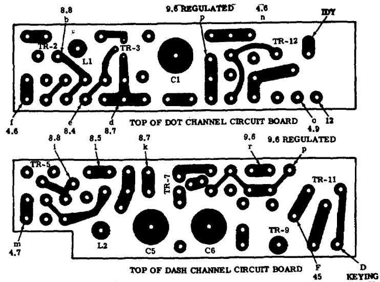
Figure 4-7. KE-3B Keyer circuit board test point diagram.
