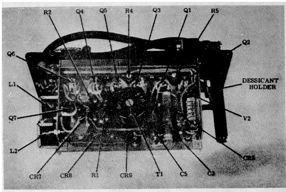
Figure 4-9. KA-3 Keyer Adapter electronics chassis, top view.
